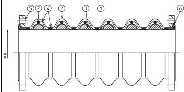
ZRJ-K400F(6山)の形状
