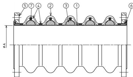
ZRJ-K300F(5山)の形状
